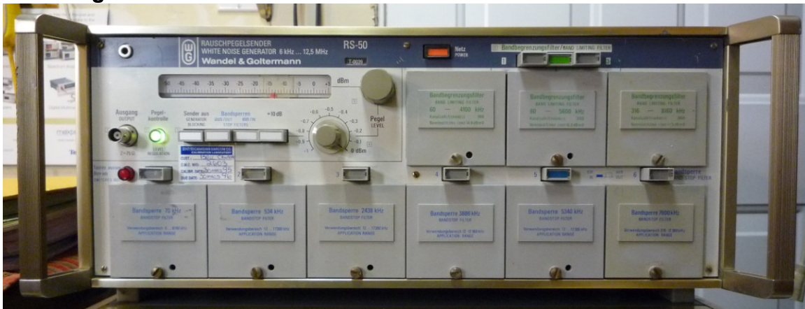
Fig.6: The Wandel & Goltermann RS-50 White Noise Generator.
