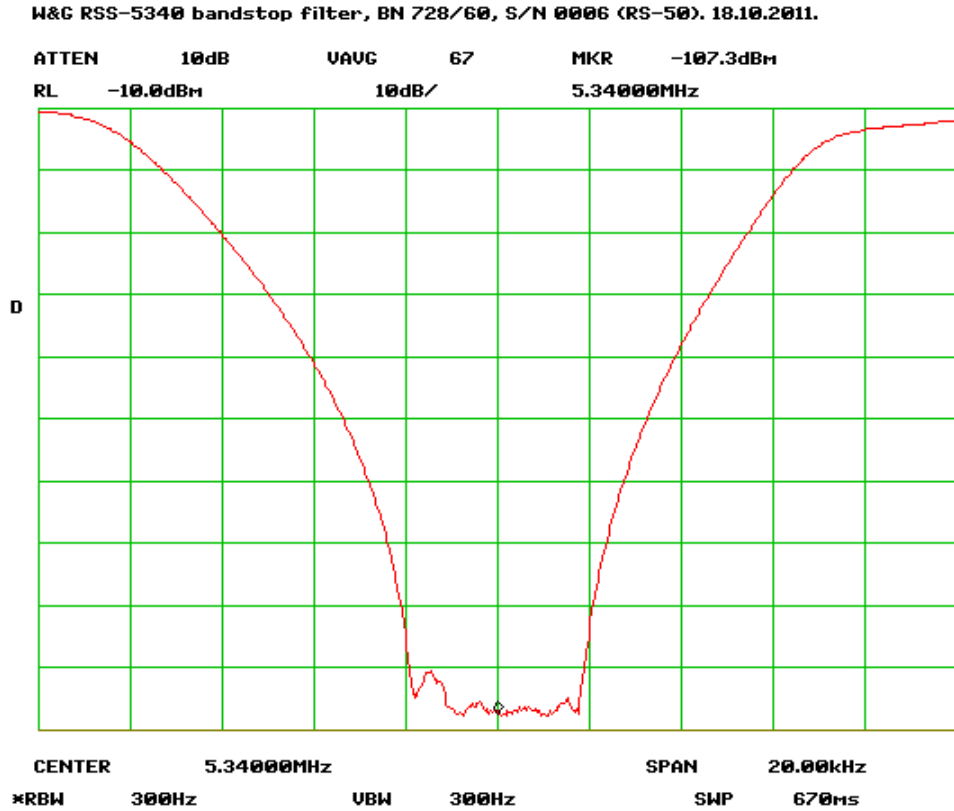
Fig.5: W&G 5340 kHz bandstop filter amplitude/frequency response.
